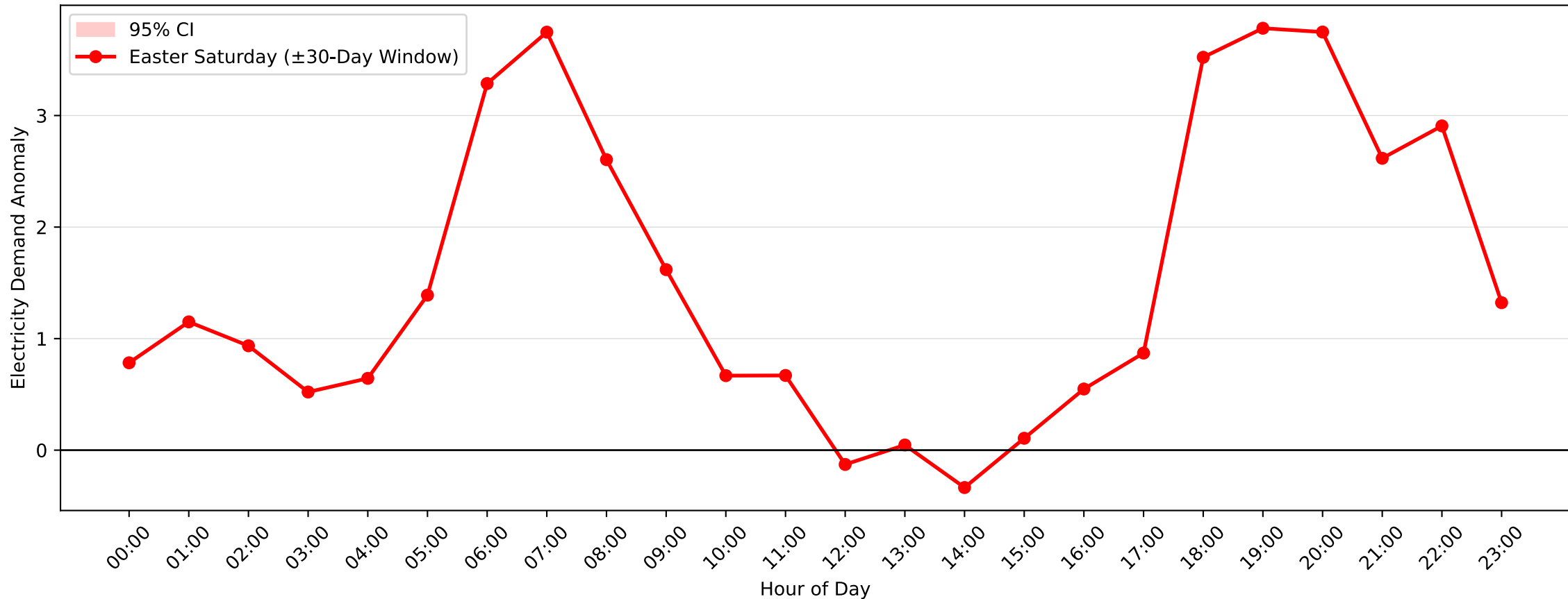
Arnccliffe Demand Anomaly: Easter Saturday (2004-2005, \pm 30 -Day Window)
