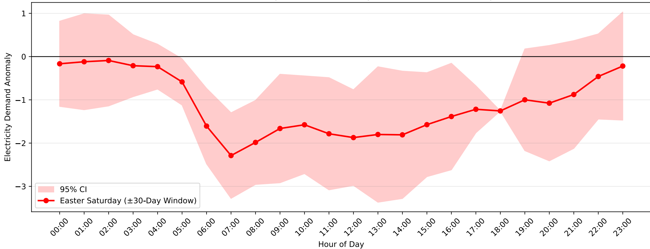
Arnccliffe Demand Anomaly: Easter Saturday (2013-2014, \pm 30 -Day Window)
