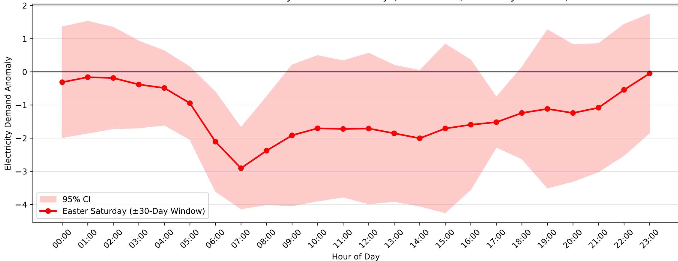
Arncliffe Demand Anomaly: Easter Saturday (2010-2011, \pm 30 -Day Window)
